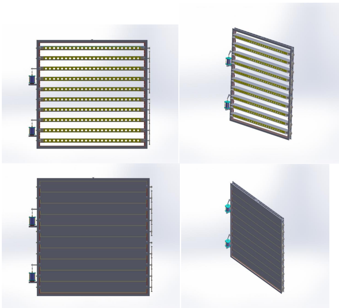
Open & Closed condition of Bi-Plane Damper
